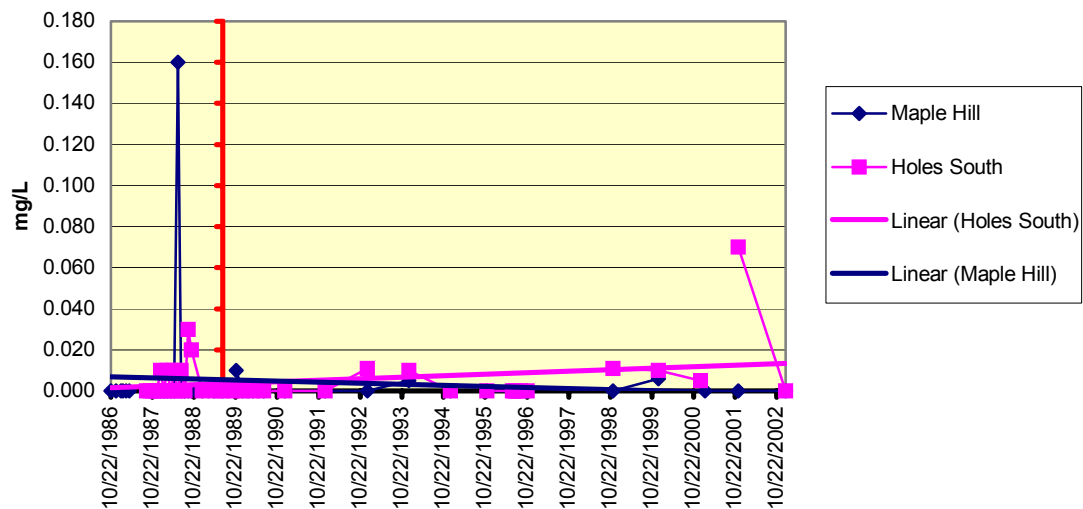
Figure 5.17 54793206-Maple Hill & Hole South-Reading Anthracite Cadmium
