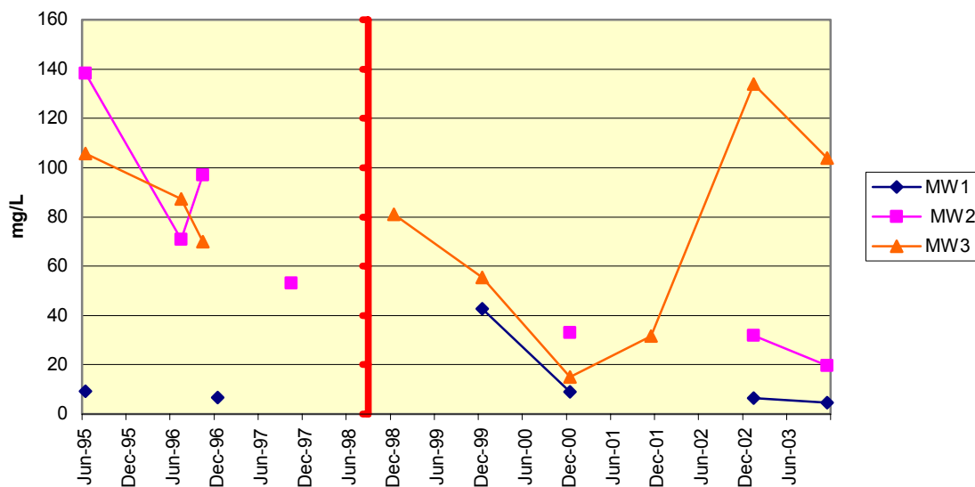
Figure 5.14 54793206-MW1 vs. MW2 & MW3-Reading Anthracite Calcium
