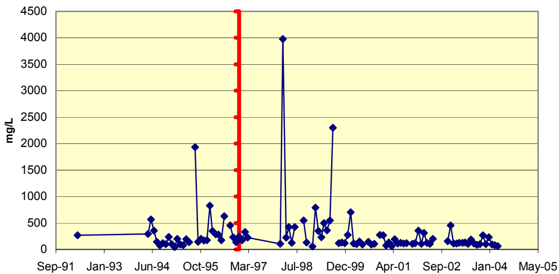
Figure 14.10 02930201 D-8 Russelton Sulfates
