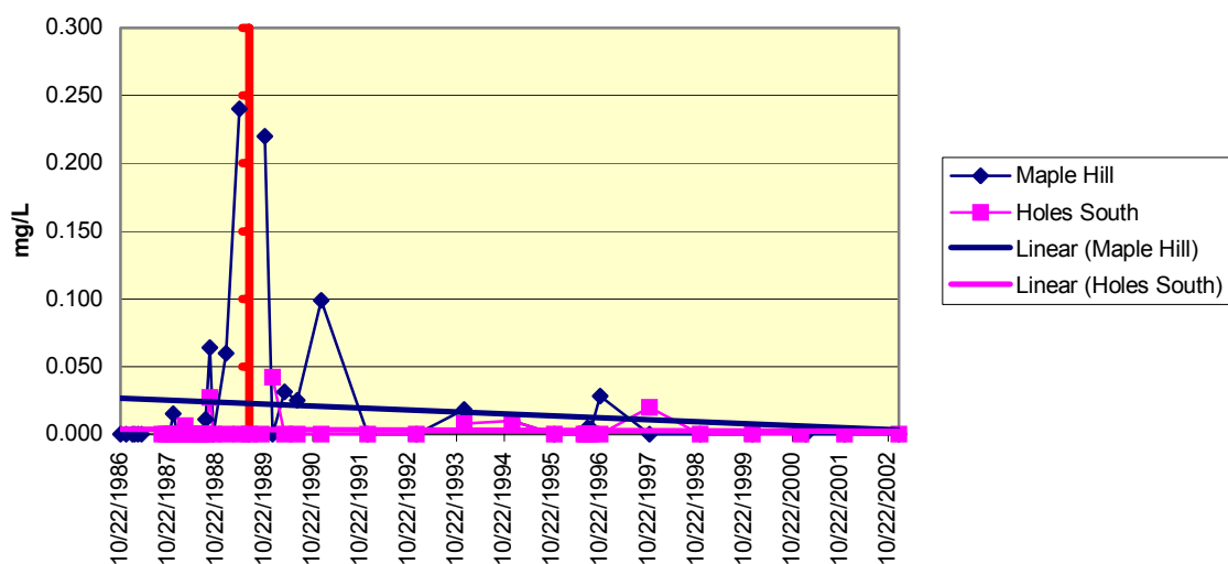
Figure 5.16 54793206-Maple Hill & Holes South-Reading Anthracite Arsenic
