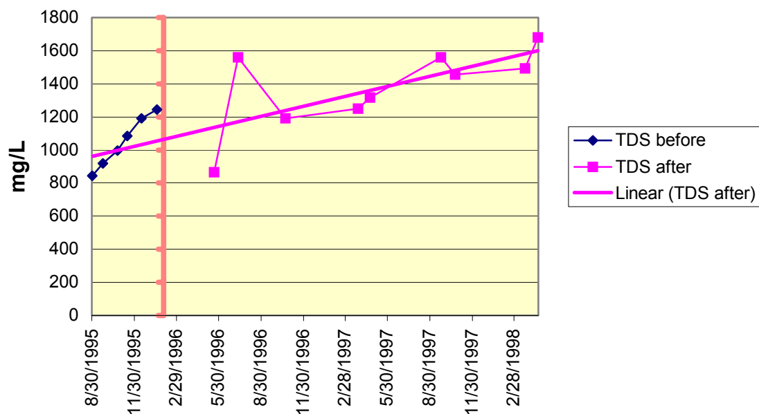
Figure 4.34 17950115 Swamp Poodle MW-4D TDS
