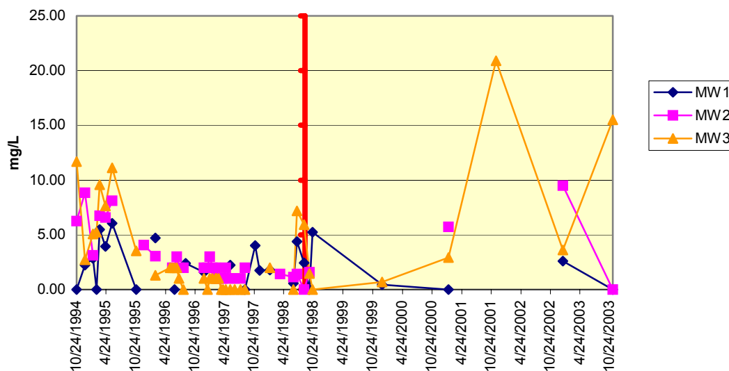
Figure 5.15 54793206-MW1vs.MW2&MW3-Reading Anthracite Chloride
