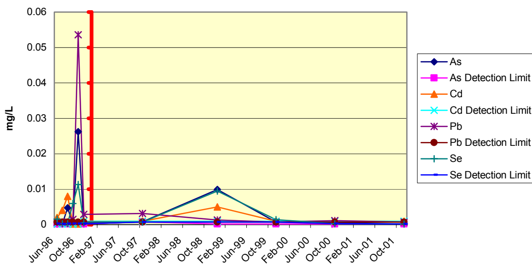
Figure 14.8 02930201 S-1d Russelton Trace Elements
