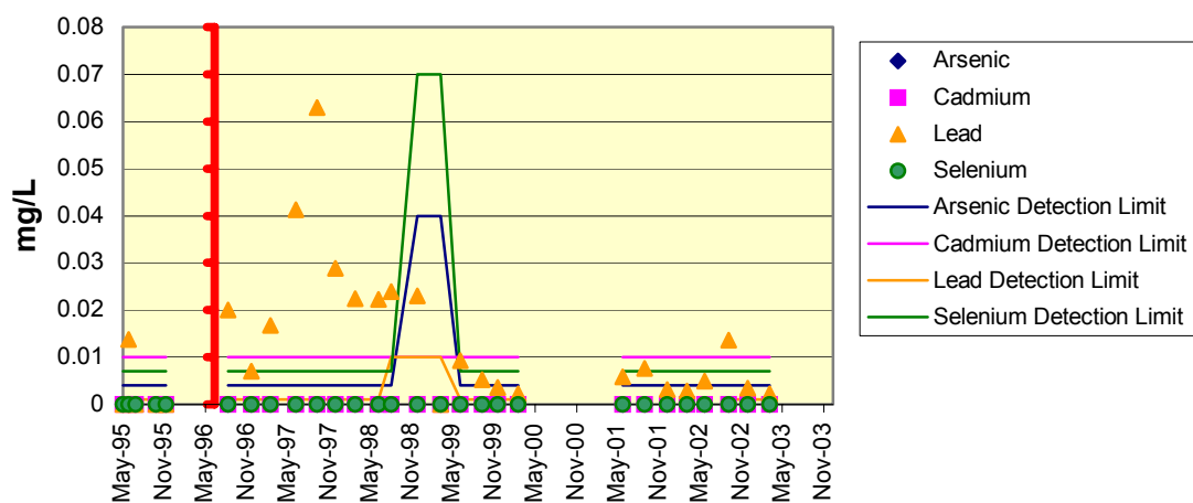
Figure 2.17 11950103-MD12-McDermott TRACE ELEMENTS
