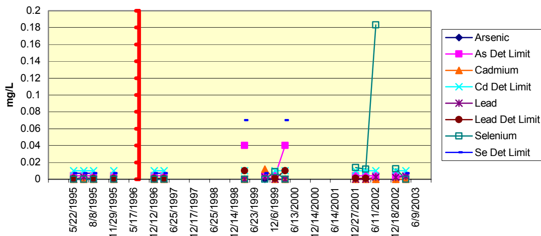
Fig. 2.31 11950102-MD19-McDermott Trace Elements
