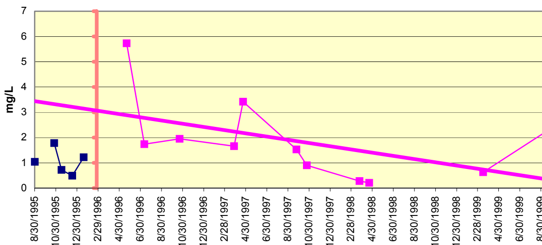
Figure 4.2 17950115 MW-1U Swamp Poodle Manganese
