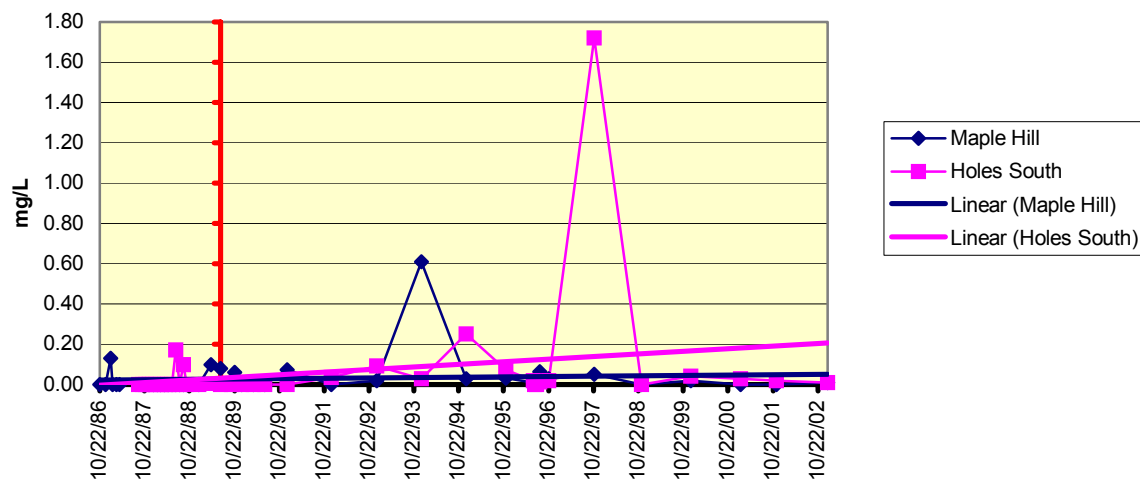
Figure 5.24 54793206-Maple Hill & Holes South-Reading Anthracite Copper
