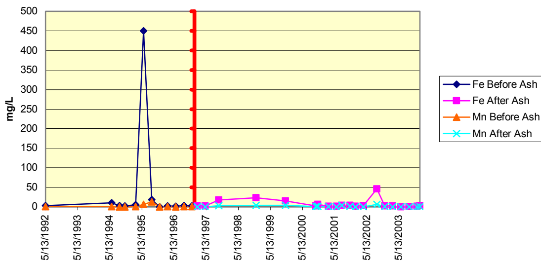
Figure 14.5 02930201 S-1d Russelton Iron & Manganese
