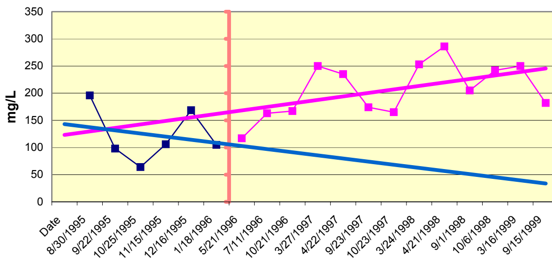
Figure 4.20 17950115 MW-3D Swamp Poodle Iron
