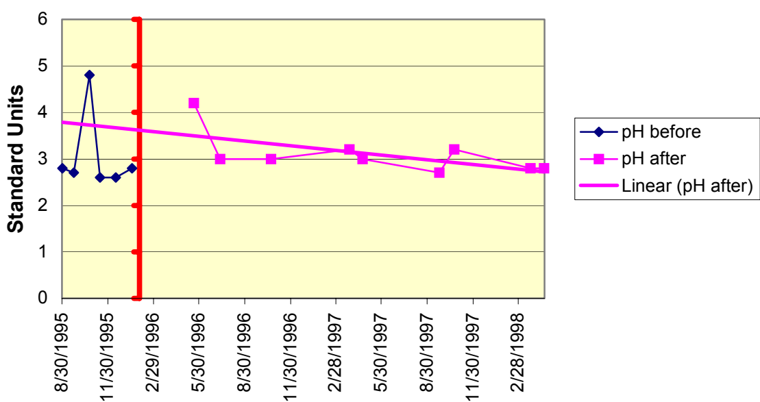
Figure 4.33 17950115 Swamp Poodle MW-4D Field pH
