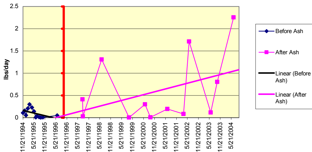
Figure 1.47 32950201 - E5 - Ernest Mine Zinc Load
