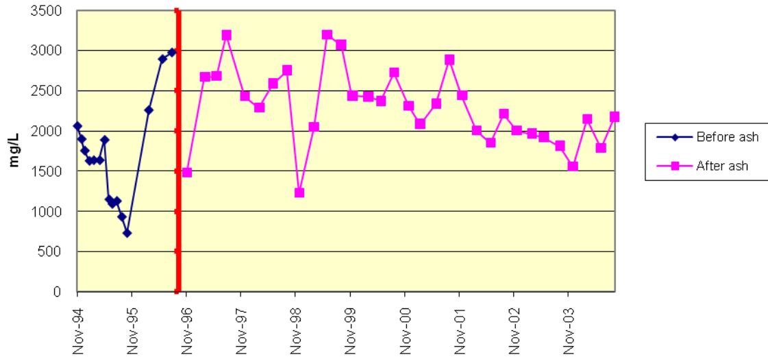
Figure 1.35 32950201-MW2-Ernest Total Dissolved Solids
