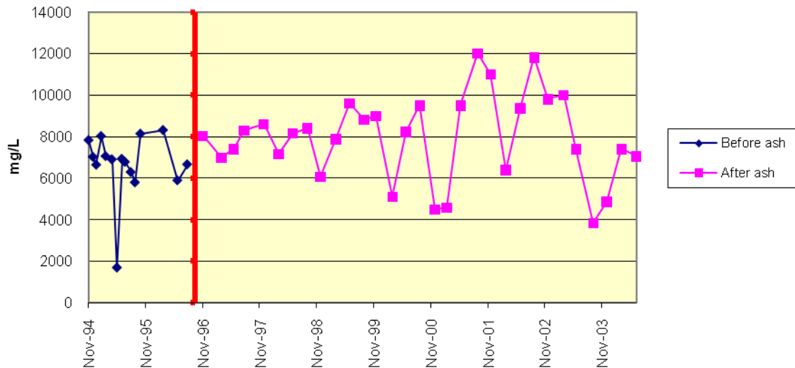
Figure 1.36 32950201-E5-Ernest Total Dissolved Solids
