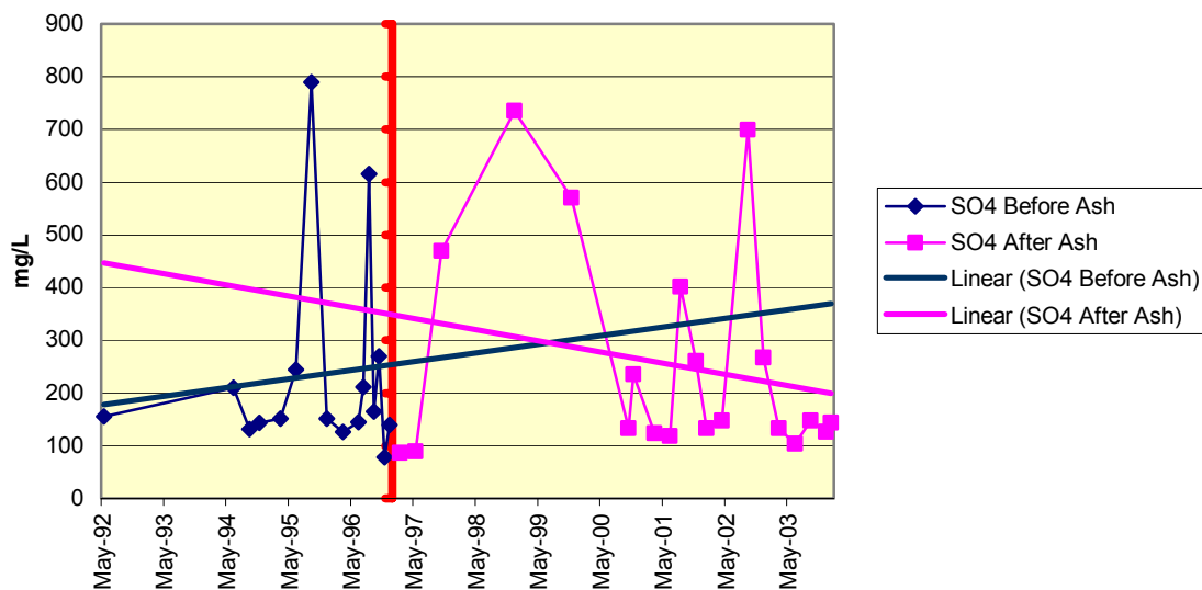
Figure 14.6 02930201 S-1d Russelton Sulfate
