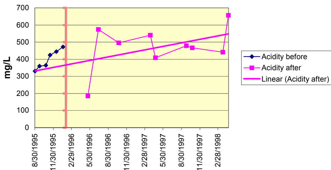
Figure 4.32 17950115 Swamp Poodle MW-4D Acidity
