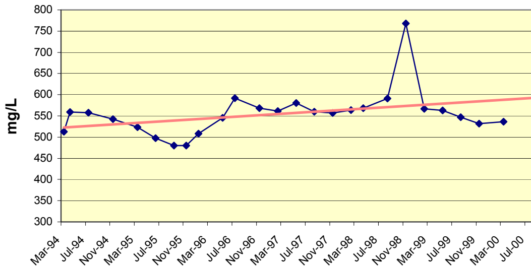
Figure 9.16A Hatfield MW-207 Alkalinity
