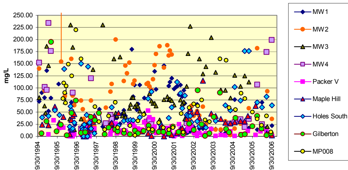
Figure 5.49b Packer V vs. Ellengowan & BD Mon. Pts. Total Suspended Solids
