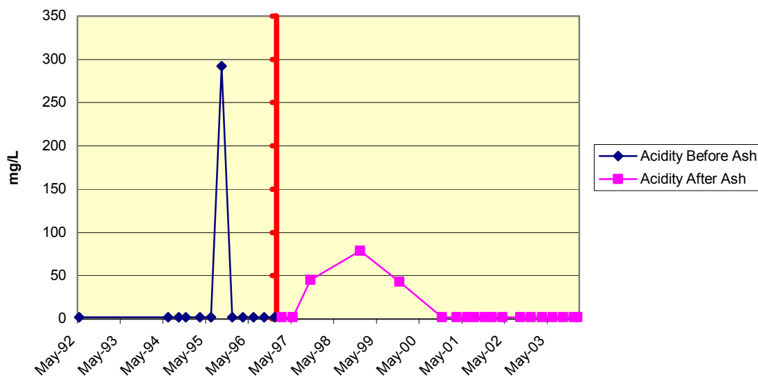
Figure 14.7 02930201 S1-d Russelton Acidity
