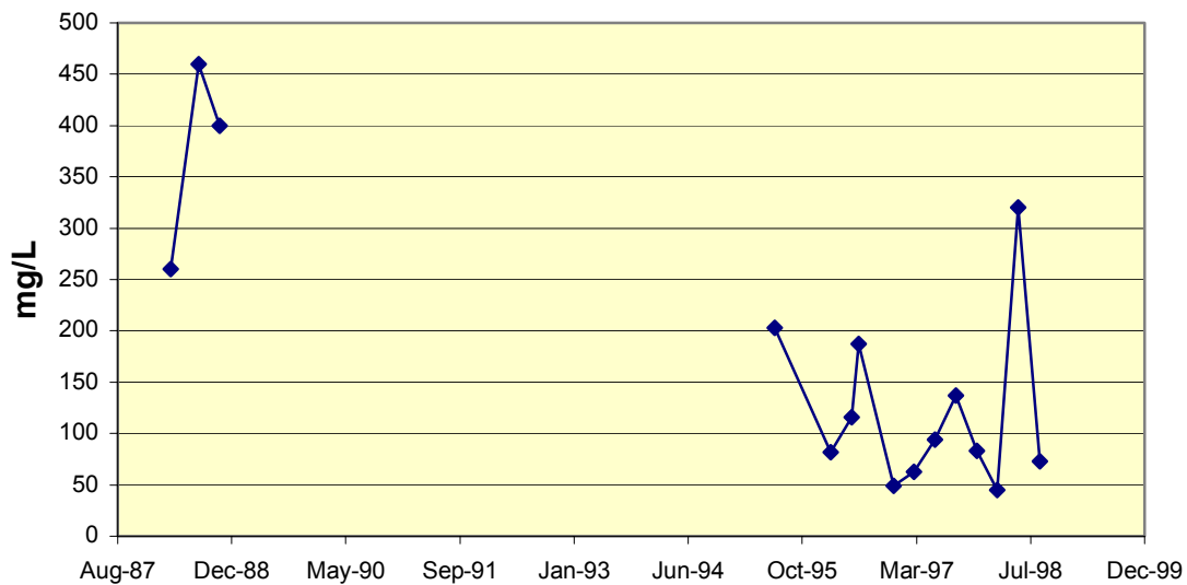
Figure 9.2 3073008 MW-1 Hartley Sulfates
