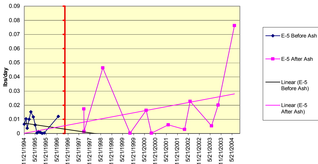
Figure 1.46 32950201 - E5 - Ernest Chromium Load
