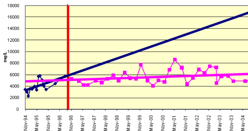
Figure 1.5 32950201-MW1-Ernest Mine SULFATES
