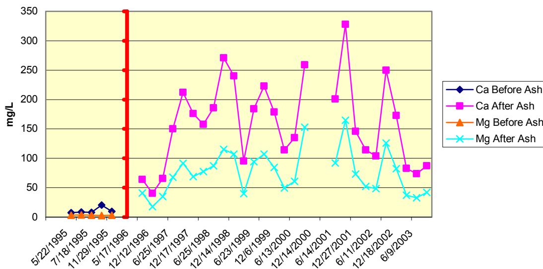
Figure 2.17a 11950102-MD12-McDermott Calcium & Magnesium
