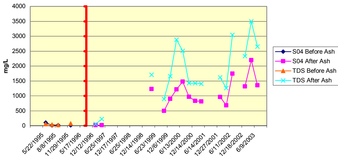
Figure 2.27 11950102-MD19-McDermott Sulfates & TDS
