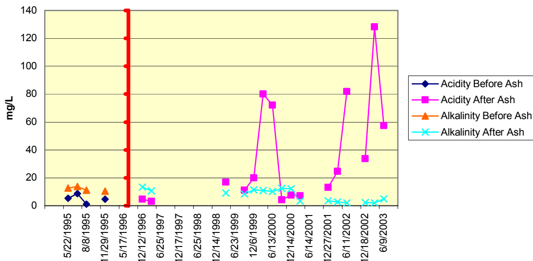
Figure 2.28 11950102-MD19-McDermott Acidity & Alkalinity
