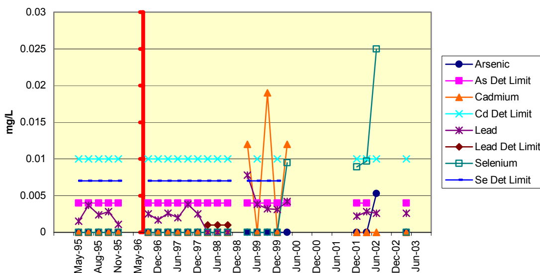
Figure 2.47 11950102-MD3-McDermott Trace Elements
