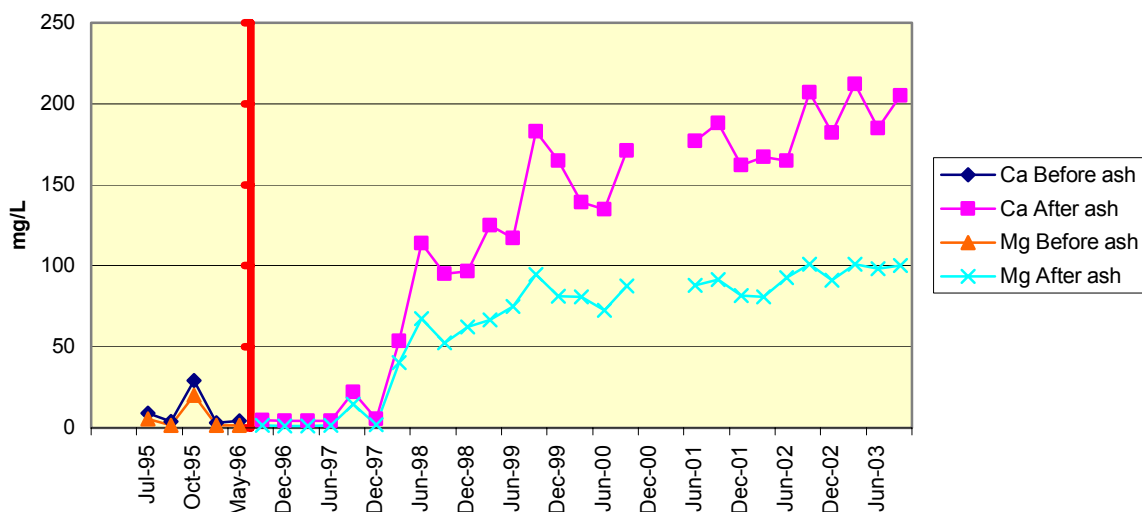
Figure 2.37 11950102-MW3-McDermott Calcium & Magnesium
