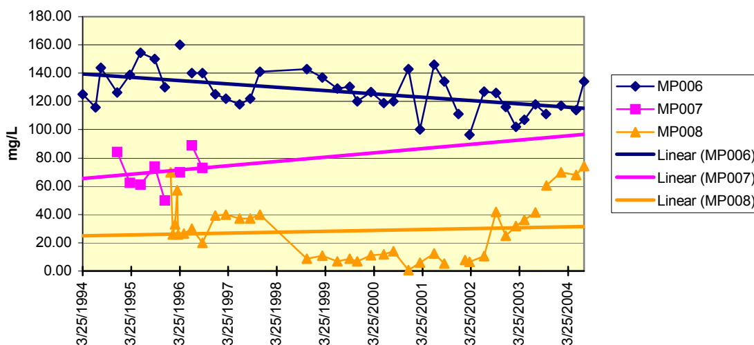
Figure 7.12 54850202-MP006vs.MP007/008-BD Mining Calcium
