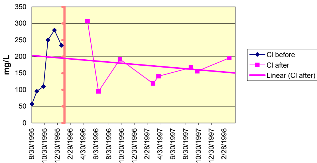
Figure 4.35 17950115 Swamp Poodle MW-4D Chloride
