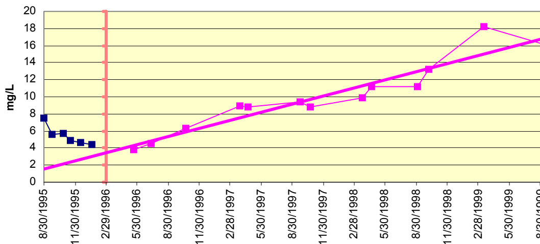
Figure 4.21 17950115 MW-3D Swamp Poodle Manganese
