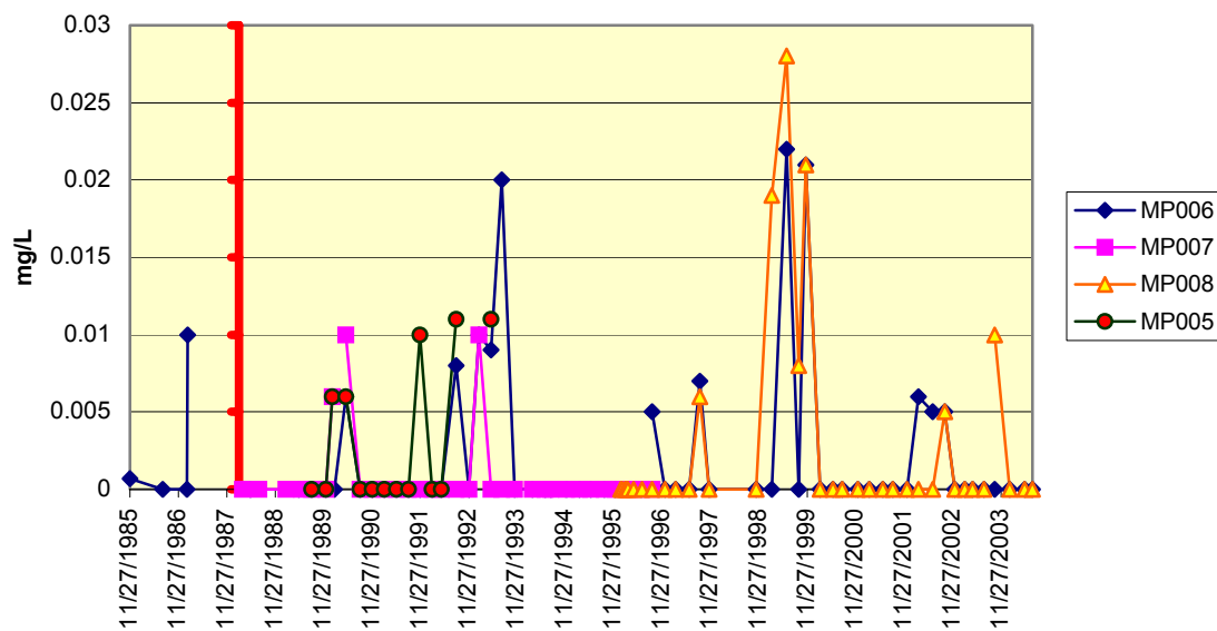
Figure 7.17 54850202-MP006vs.MP007/008/005-B-D Mining Cadmium
